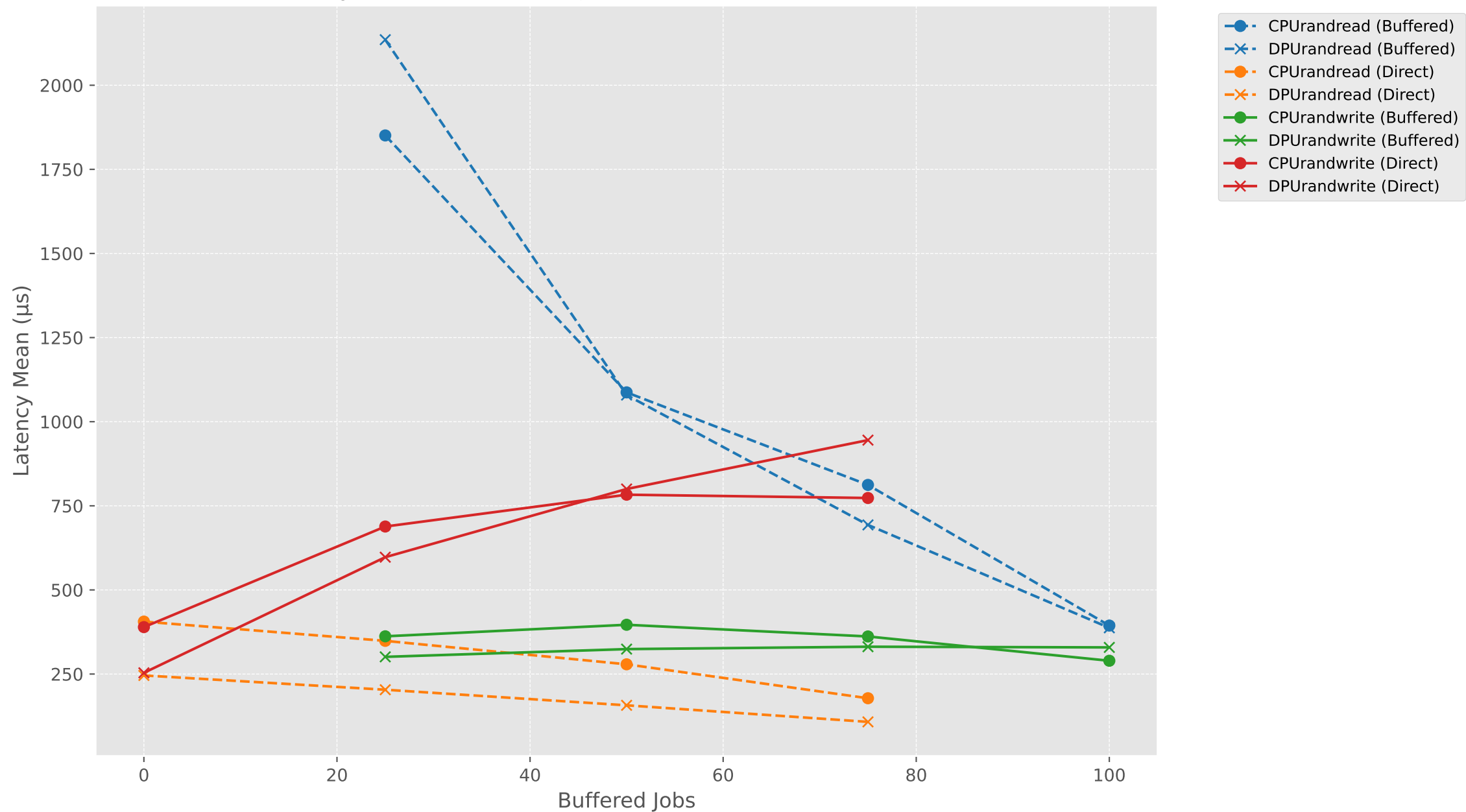
Latency Mean vs Buffered Jobs (mixed) - RAND (CPU vs DPU)
